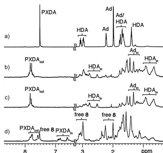
Figure 9. 1 H NMR spectra (400 MHz, D 2 O, rt) recorded for: (a) 8 , and mixtures of bis- ns -CB[10] and 8 at different relative stoichiometries (b) 1:1, (c) 2:1, and (d) 1:2.
