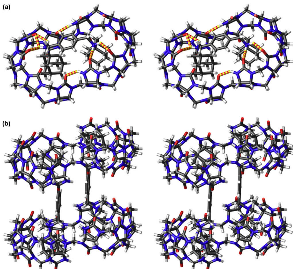
Figure 5. Stereoviews of the MMFF minimized geometries of: (a) bis-ns-CB[10]· 1 and (b) bis-ns-CB[10] 2 · 4 2 . Color code: C, gray; H, white; N, blue; O, red; H-bonds, red-yellow stripped.
