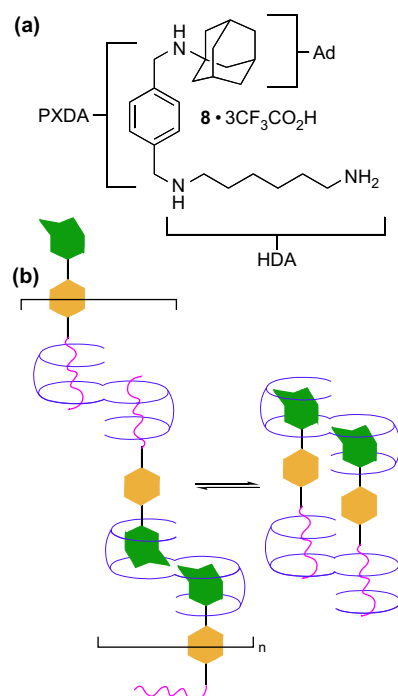
Figure 8. (a) Depiction of the three binding domains of 8 along with their abbreviations used in this paper. (b) Theoretical equilibrium between a linear polymer comprising bis- ns -CB[10] and 8 and bis- ns -CB[10] 2 · 8 2 .
