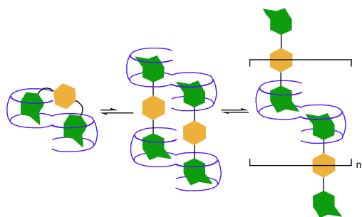
Figure 4. Potential equilibrium between bis-ns-CB[10]·1, bis-ns-CB[10] 2 ·1 2 , and bis-ns-CB[10] n ·1 n complexes.
