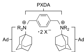
Figure 2. Depiction of the two different binding domains of the xylene derived guests ( 1 , 2 , and 4–6 ) along with their abbreviations used in this paper.
