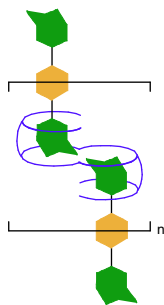
Figure 1. Hypothetical linear polymer comprising bis-ns-CB[10] and 1 .
