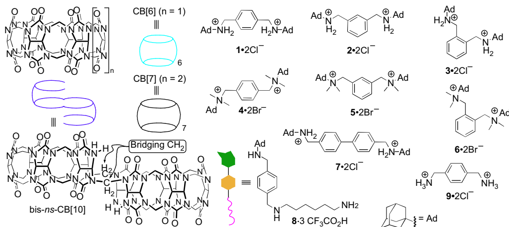
Chart 1. Compounds used in this study.
