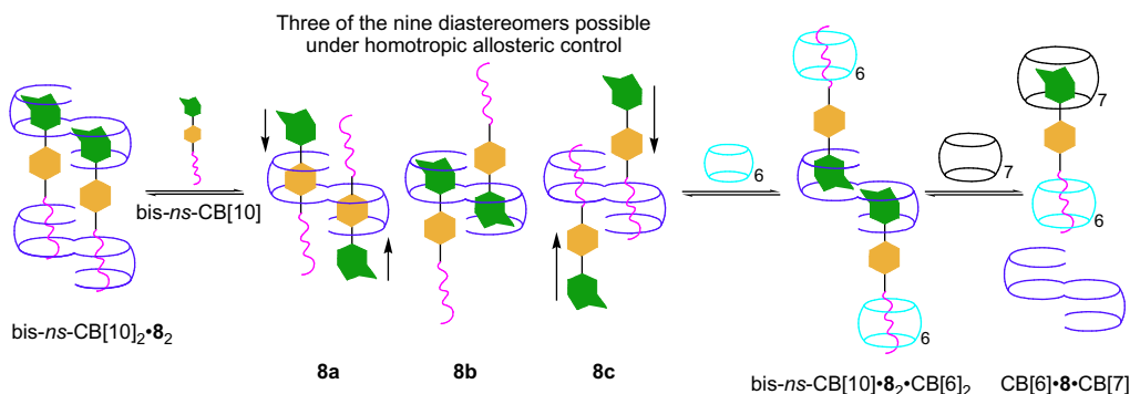
Scheme 3. Depiction of the equilibrium structures obtained upon treatment of bis-ns-CB[10] 2 ·8 2 with 8 then CB[6] then CB[7].
