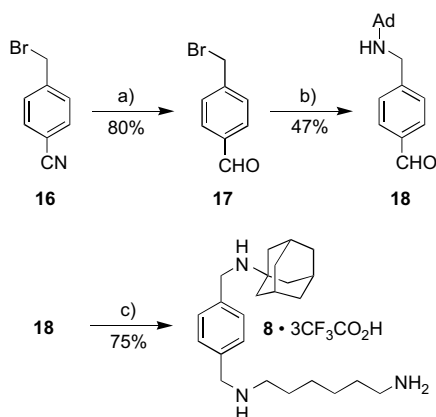
Scheme 2. Synthesis of 8 . Reaction conditions: (a) (i) DIBAL, toluene, 0 °C, 1 h, (ii) 10% HCl, 1 h, rt, (b) 10 , Ag 2 O, THF, (c) (i) N -( tert -butoxycarbonyl)-1,6-hexanediamine ( 19 ), toluene, reflux, 20 h, (ii) NaBH 4 , MeOH, reflux (30 min), then stir at rt (15 h), (iii) TFA/CH 2 Cl 2 (1:1), rt, 8 h.
