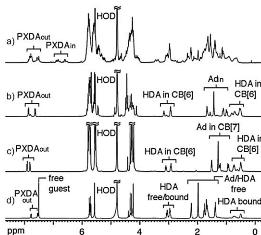
Figure 11. 1 H NMR spectra (400 MHz, D 2 O, rt) recorded for solutions of: (a) bis-ns-CB[10]·8 2 , (b) after addition of 2 equiv CB[6] to obtain CB[6] 2 ·8 2 ·bis-ns-CB[10], and (c) after addition of 2 equiv CB[7] to obtain CB[7]·8·CB[6] and solid bis-ns-CB[10]. (d) Control spectrum for a mixture of CB[6]· 8 and excess 8 .
