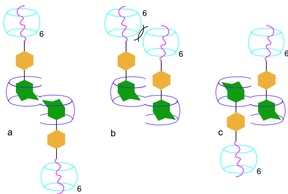
Figure 12. Three different diastereomers of the bis- ns -CB[10]·8 2 ·CB[6] 2 complex.
