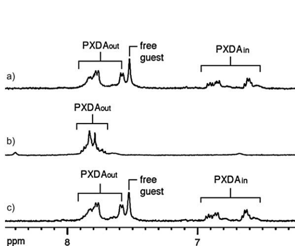
Figure 10. Aromatic region of the 1 H NMR spectra (400 MHz, D 2 O, rt) of a sample undergoing alternate successive additions of bis-ns-CB[10] and 8 : (a) a 1:2 ratio of bis-ns-CB[10] to 8 , (b) after addition of excess bis-ns-CB[10], and (c) after addition of excess 8 .
