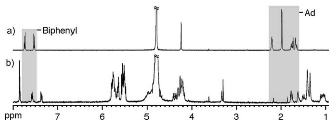
Figure 6. 1 H NMR spectra (400 MHz, D 2 O, rt) recorded for solutions of: (a) 7 , (b) bis- ns -CB[10] 2 · 7 2 .
