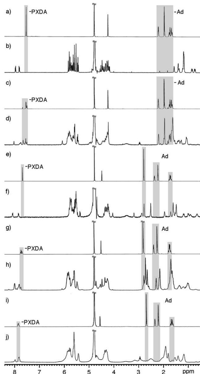
Figure 3. 1 H NMR spectra (400 MHz, D 2 O, rt) recorded for solutions of: (a) 1 , (b) bis-ns-CB[10]· 1 , (c) 2 , (d) a mixture of 2 and bis-ns-CB[10]· 2 , (e) 4 , (f) a mixture of 4 and bis-ns-CB[10]· 4 , (g) 5 , (h) a mixture of 5 and bis-ns-CB[10]· 5 , (i) 6 , (j) bis-ns-CB[10]· 6 .
