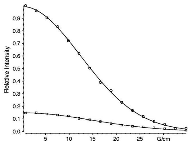
Figure 7. Plot of signal intensity versus gradient strength and the best fit of the data to Eq. 1. Symbols: ○, bis- ns -CB[10] 2 · 7 2 ; □, bis- ns -CB[10]· 9 2 .
