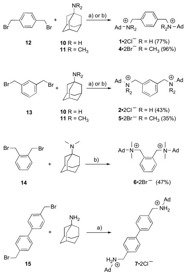
Scheme 1. Synthesis of guest compounds 1 , 2 , and 4–7 . Conditions: (a) Ag 2 O, THF; (b) CH 3 CN, reflux.
